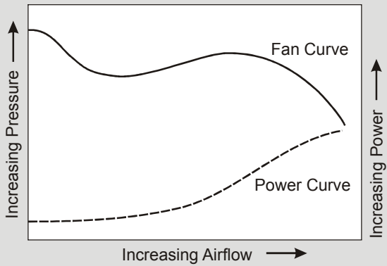
Forward Curved
