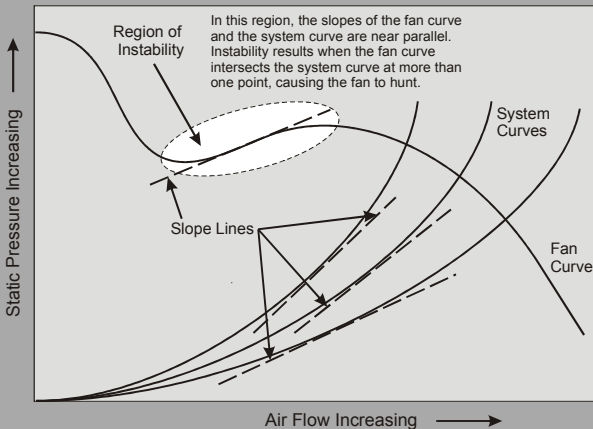
Figure 10: Fan Curve with Instability Zone
