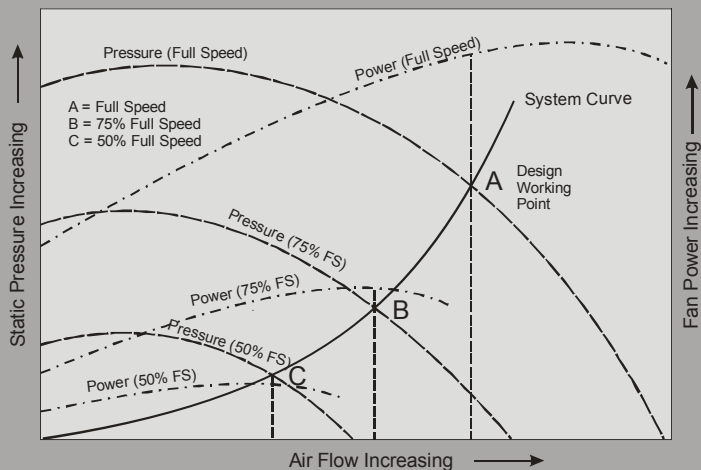
Figure 13: Flow Control by Speed Regulation
