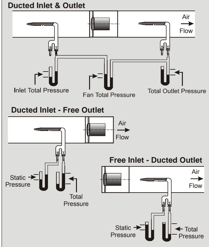
Figure 19: Alternative Methods of Measuring Fan Pressure
